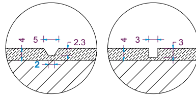
Birdsmouth Joint
