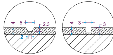
Birdsmouth Joint
